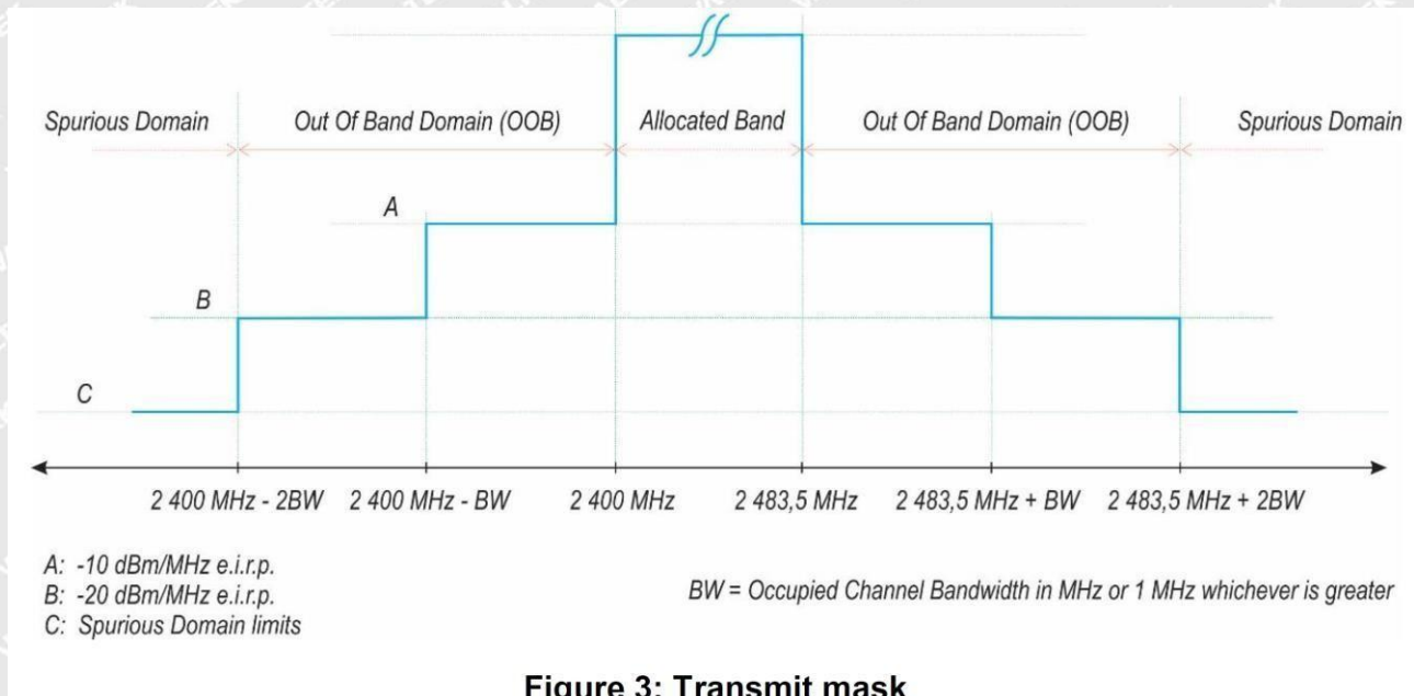
Figure 3: Transmit mask
